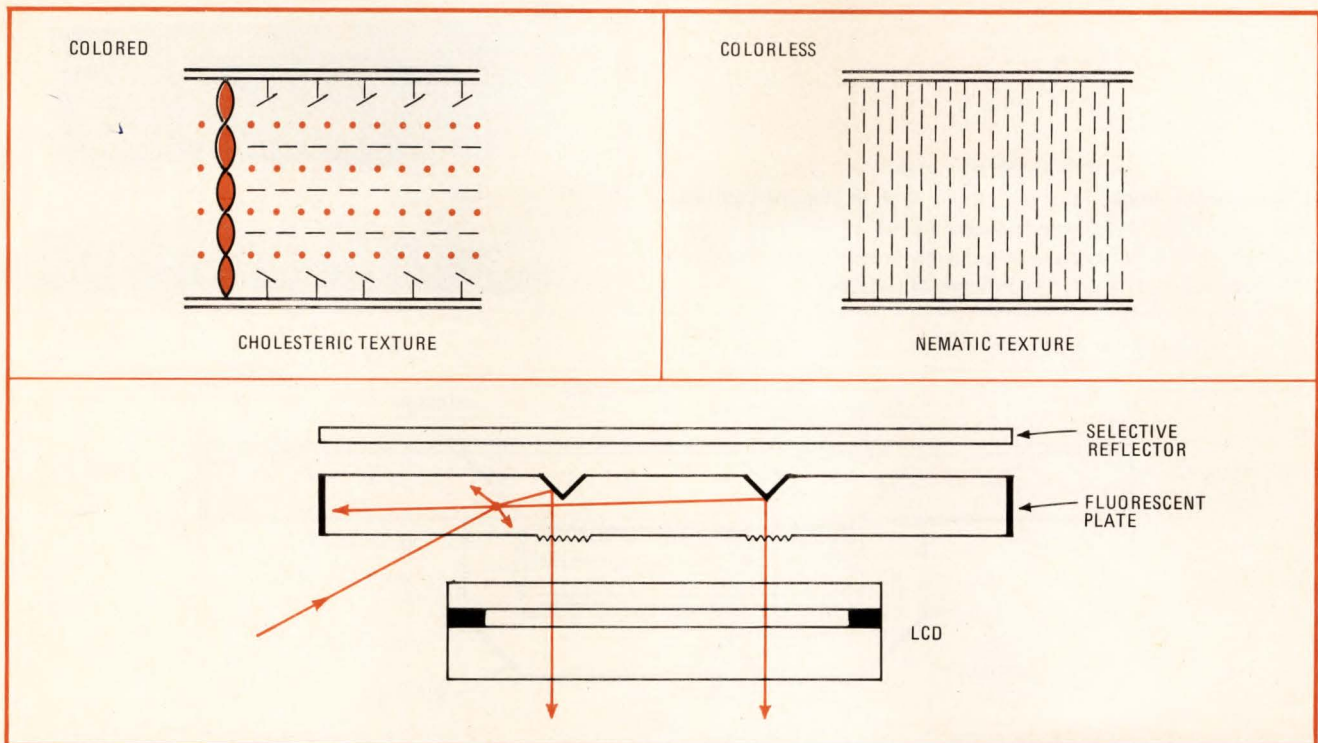
4. Colored LCD. Pleochroic-dye displays (top left) have a twisted-nematic material (top right) that reorients molecules of the dye so that a white numeral is shown on a colored background. With this type of display, the FLAD (bottom) requires no polarizers.
