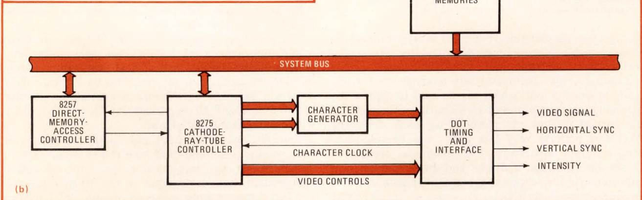
4. Controlling cathode-ray tubes. In CRT controllers such as Intel's 8275, the character counter determines the number of characters to be displayed and the length of the retrace interval. The system (b) is driven by a direct-memory-access controller.
