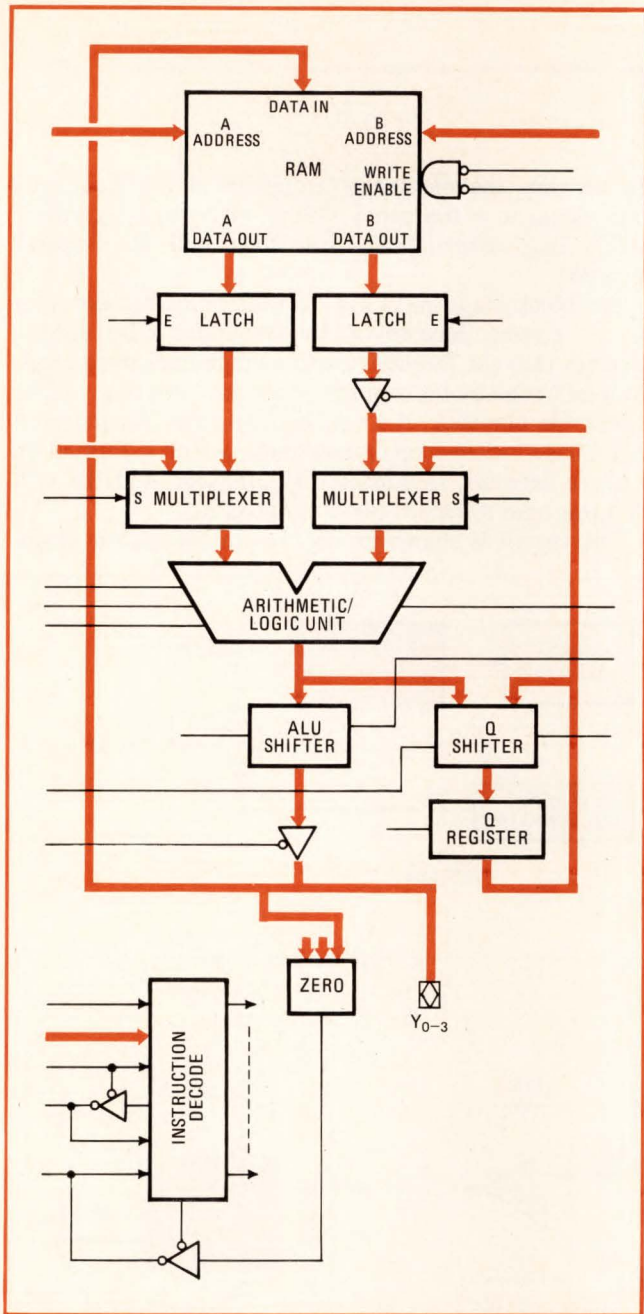
7. Simpler still. The next-generation 2903 bit-slice microcomputer, besides performing better, is easier to design with, especially in arithmetic-oriented systems. Memory can be expanded indefinitely, and a three-address architecture gives maximum flexibility.
