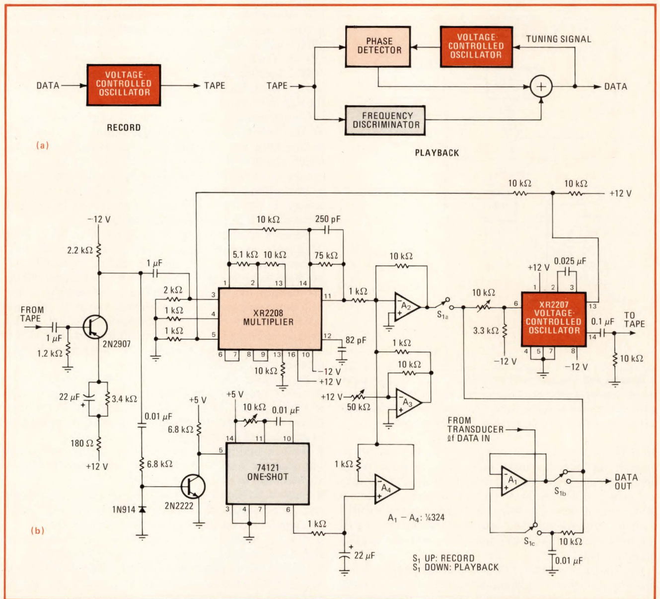
Data translation. Low-frequency data may be recorded on an inexpensive tape recorder if the signal is first modulated to a higher frequency. Signal is recovered from recorder by demodulation, using same VCO (a). Modulator uses four chips and two transistors (b).
