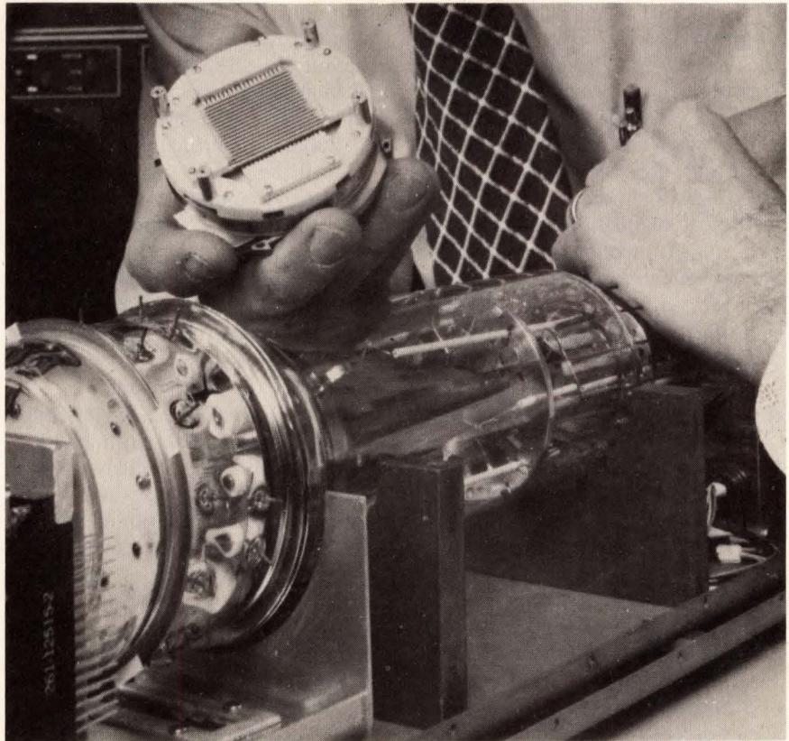
Beamos. Once it is placed inside a GE memory tube, the array of tiny lenses focuses electron beams onto information storage sites contained in a metal-oxide-semiconductor target.
